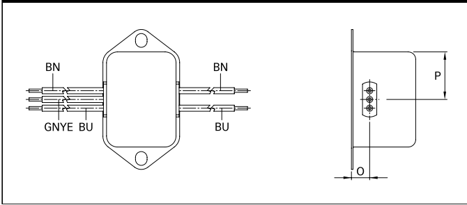
Connection style -07, 1 to 12 A types (same dimensions as style -06)
